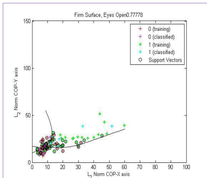
Figure 2: Svm: Training And Classification: Condition EO: Effect Of Dyskinesia: On Medication.
